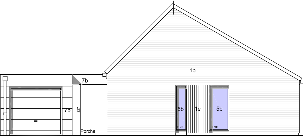
FACADE RUE
