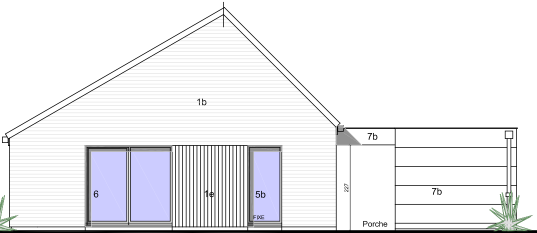
FACADE PIGNON JARDIN
