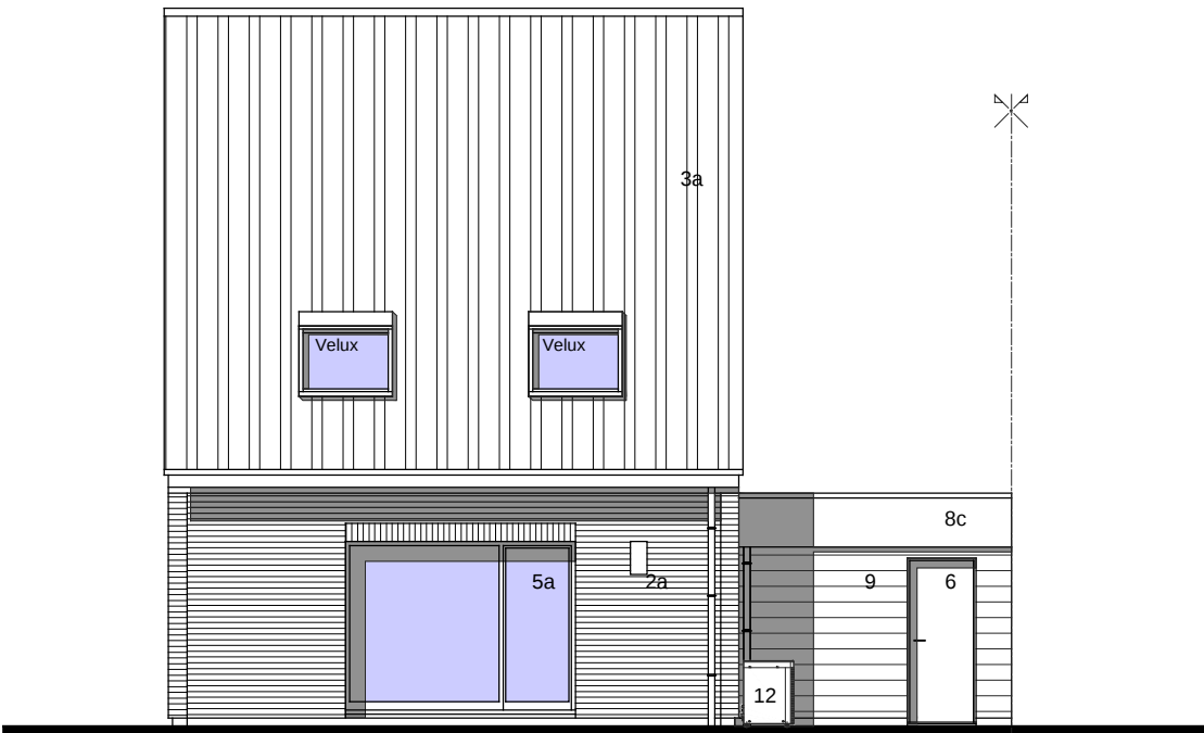
FACADE ARRIERE
